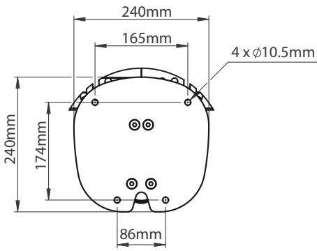
BASE PLATE
